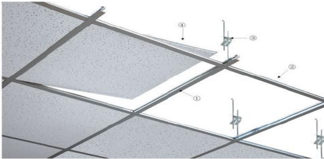
① Main tee ② Cross tee ③ Hanger for T-grid ④ Mineral fiber tile
